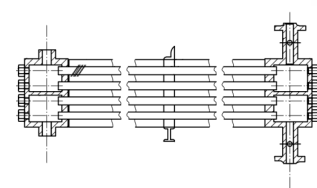
Plug-type Collector
